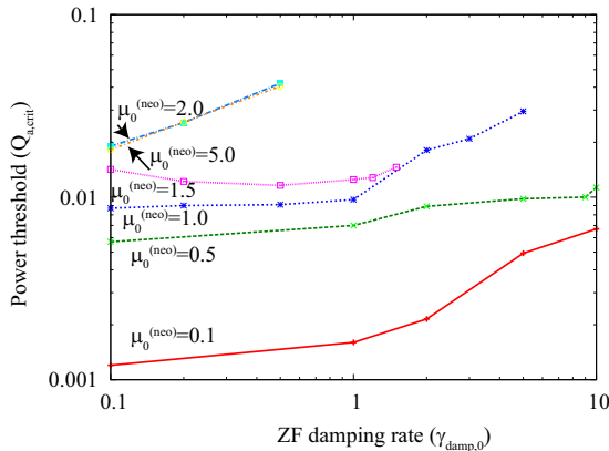
FIG. 13. Investigation of power threshold Q_{a,crit} for various ZF damping rates \gamma_{damp} as well as for neoclassical poloidal flow viscosities \mu_0^{(neo)} . In cases with \mu_0^{(neo)} \geq 2.0 , no transition occurs for Q_a < 0.05 . In case of \mu_0^{(neo)} = 1.5 and \gamma_{damp} > 2.0 , the transition does not occur for Q_a < 0.05 . In cases with \mu_0^{(neo)} = 1.0 and \gamma_{damp} > 1.0 , the transition does not occur for Q_a < 0.05 . In case of \mu_0^{(neo)} = 0.5 , and \gamma_{damp} = \infty , i.e., without ZF shearing ( \alpha_0 = 0 ), the transition occurs at Q_a = 0.013 . In case of \mu_0^{(neo)} = 0.1 , without ZF shearing, the transition occurs at Q_a = 6.7 \times 10^{-3} , which power threshold is equivalent to the case of \mu_0^{(neo)} = 0.1 and \gamma_{damp} = 1.0 .
